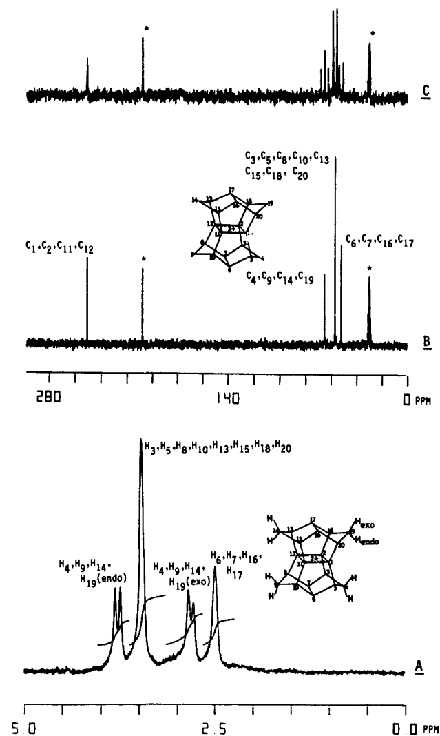
Figure 1. (A) 200-MHz ^1\text{H} NMR spectrum of pagodane dication in \text{SbF}_5/\text{SO}_2\text{ClF} solution at -80^\circ\text{C} . (B) 50-MHz proton-decoupled ^{13}\text{C} NMR spectrum. (C) Proton-coupled spectrum (* peaks due to lock solvent (\text{CD}_3)_2\text{CO} ).
